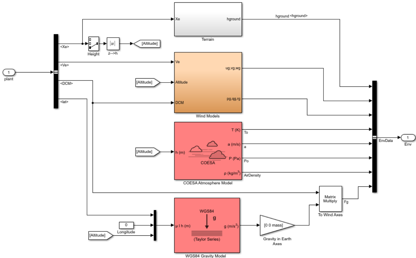
Figure 8: Environmental effect of wind, atmosphere, and gravity using Aerospace Blockset blocks.
